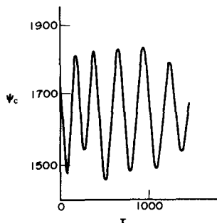
FIG. 13. Steady oscillations of the central stream function for Ra = 6.3 \times 10^{10} , Pr = 6.7 and \Delta\tau = 1 \sim 3 .
