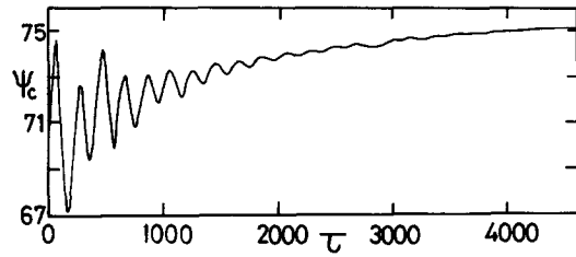
FIG. 7. Transient response of the dimensionless central stream function for Ra = 1.52 \times 10^8 and Pr = 9.17 with \Delta\tau = 0.1 to 0.2.
