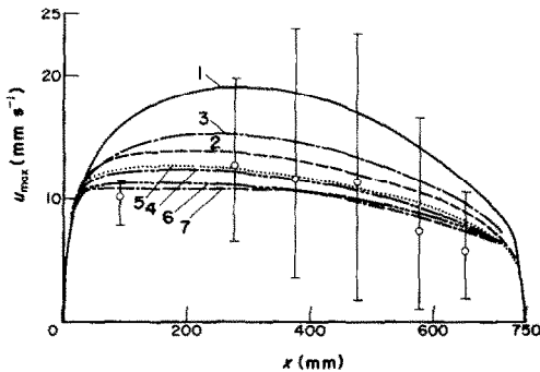
FIG. 20. Comparison for Ra = 6.26 \times 10^{10} and Pr = 5.12 of the computed peak vertical velocities over the heated vertical wall of a square enclosure with the experimental oscillating velocities at the displacement corresponding to the peak velocity.
