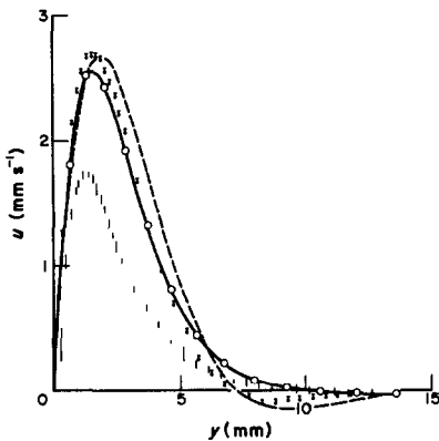
FIG. 10. Comparison for Ra = 1.52 \times 10^8 and Pr = 9.17 of the computed vertical velocities with experimental values in a 160 mm high, 295 mm wide and 189 mm deep enclosure. —○— Measured vertical velocity at x = 15 mm —○— Measured vertical velocity at x = 75 mm —○— Computed vertical velocity at a height equivalent to x = 15.8 mm --- Computed vertical velocity at a height equivalent to x = 80 mm.
