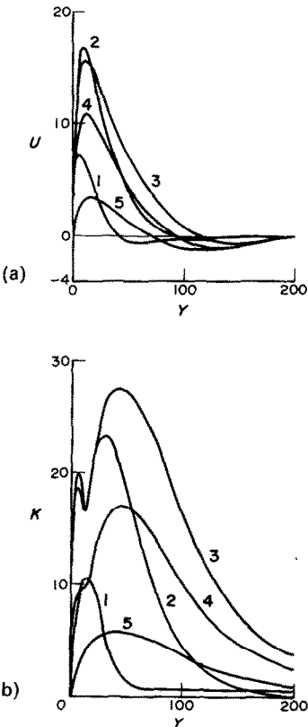
FIG. 21. Computed vertical velocity profiles, (a) and turbulent kinetic energy K_{10} (b) at various heights. Ra = 6.3 \times 10^{10} , Pr = 6.7 , \sigma_t = 4 and c_1 = 1.296 ( -10\% ).
