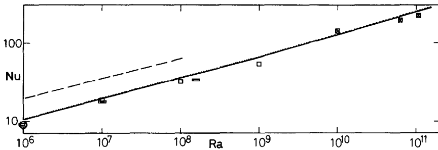
FIG. 9. Comparison of the computed overall Nusselt number with correlating equation of Churchill [12] for L/H = 1 and 2. L/H = 2 □ Laminar model — Correlating equation L/H = 1 □ Laminar model ⊗ Turbulent model ---- Correlating equation ○ Comparison problem report [15] ---- Correlating equation for vertical plate in unconfined fluid [13].
