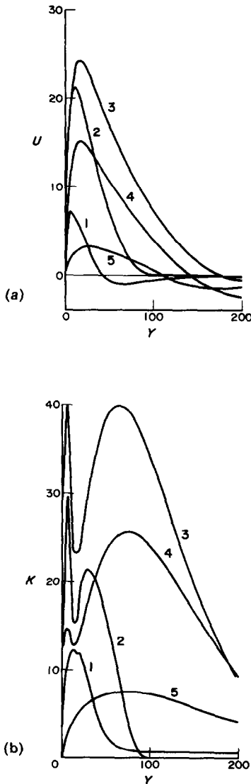
FIG. 16. Computed results for Ra = 6.3 \times 10^{10} and Pr = 6.7 with standard set of constants in k-\epsilon model. (a) Profiles of dimensionless vertical velocity at various heights; (b) profiles of dimensionless turbulent kinetic energy at various heights.
