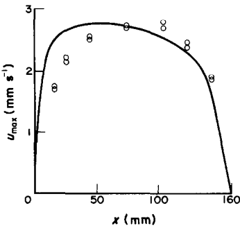
FIG. 11. Comparison of computed peak vertical velocities for L/H = 2 , Ra = 1.52 \times 10^8 and Pr = 9.17 with experimental values. — Computed ○ Range of fluctuation of experimental peak velocities in 160 mm high, 295 mm wide and 189 mm deep enclosure.
