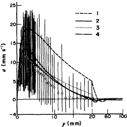
Fig. 17. Comparison of computed and experimental vertical velocities along the heated wall of a square enclosure for Ra = 6.26 \times 10^{10} , Pr = 6.3 and x = 37.5 cm. The experimental box is 750 mm \times 750 mm \times 180 mm.
