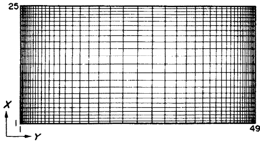
FIG. 2. Example of grid point distribution for L/H = 2 .
