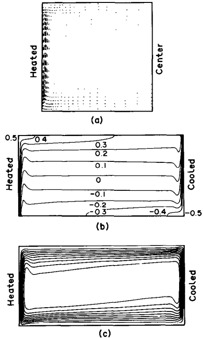
FIG. 5. Steady state solution for Ra = 10^7 and Pr = 9.17 . (a) Velocity vectors; (b) dimensionless isotherms; (c) streamlines.
