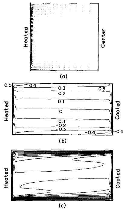
FIG. 8. Steady state solution for Ra = 1.52 \times 10^8 and Pr = 9.17 using the hybrid scheme of Patankar [11]. (a) Velocity vectors; (b) dimensionless isotherms; (c) streamlines.
