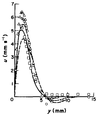
Fig. 12. Comparison of the vertical velocity near the heated vertical wall with experimental measurements in water by laser-Doppler velocimetry. Computed condition: Ra = 10^9 , Pr = 5.12 , x = 43.2 mm —, x = 105 mm ---, x = 166.8 mm ——. Experimental condition: Ra = 1.04 \times 10^9 , Pr = 5.12 , x = 45 mm \square , x = 105 mm \triangle , x = 165 mm \circ .
