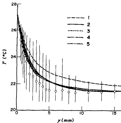
FIG. 19. Comparison of computed temperature profiles at mid-height for various combinations of constants in the k - \epsilon model with the experimental measurements.
