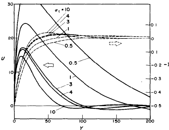
FIG. 18. Profiles of dimensionless vertical velocity and temperature at middle height for various values of the turbulent Prandtl number \sigma_t . Ra = 6.3 \times 10^{10} and Pr = 6.7 .
