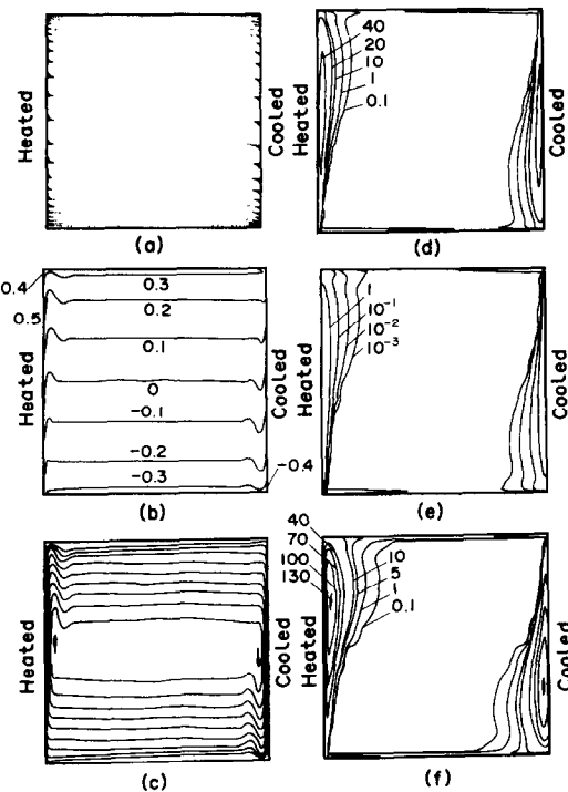
FIG. 15. Contour maps for the computed time-averaged characteristics of turbulent natural convection at Ra = 1.09 \times 10^{11} and Pr = 6.7 in a square channel. (a) to (f) are the same as in Fig. 14.
