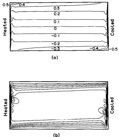
FIG. 6. Steady state solution for Ra = 10^8 and Pr = 9.17 . (a) Dimensionless isotherms; (b) streamlines.
