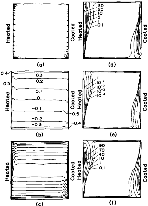
FIG. 14. Contour maps for the time-averaged characteristics of turbulent natural convection at Ra = 6.3 \times 10^{10} and Pr = 6.7 in a square channel. (a) Velocity vectors; (b) dimensionless isotherms; (c) streamlines; (d) turbulent kinetic energy; (e) rate of dissipation of turbulent energy; (f) dimensionless eddy diffusivity.
